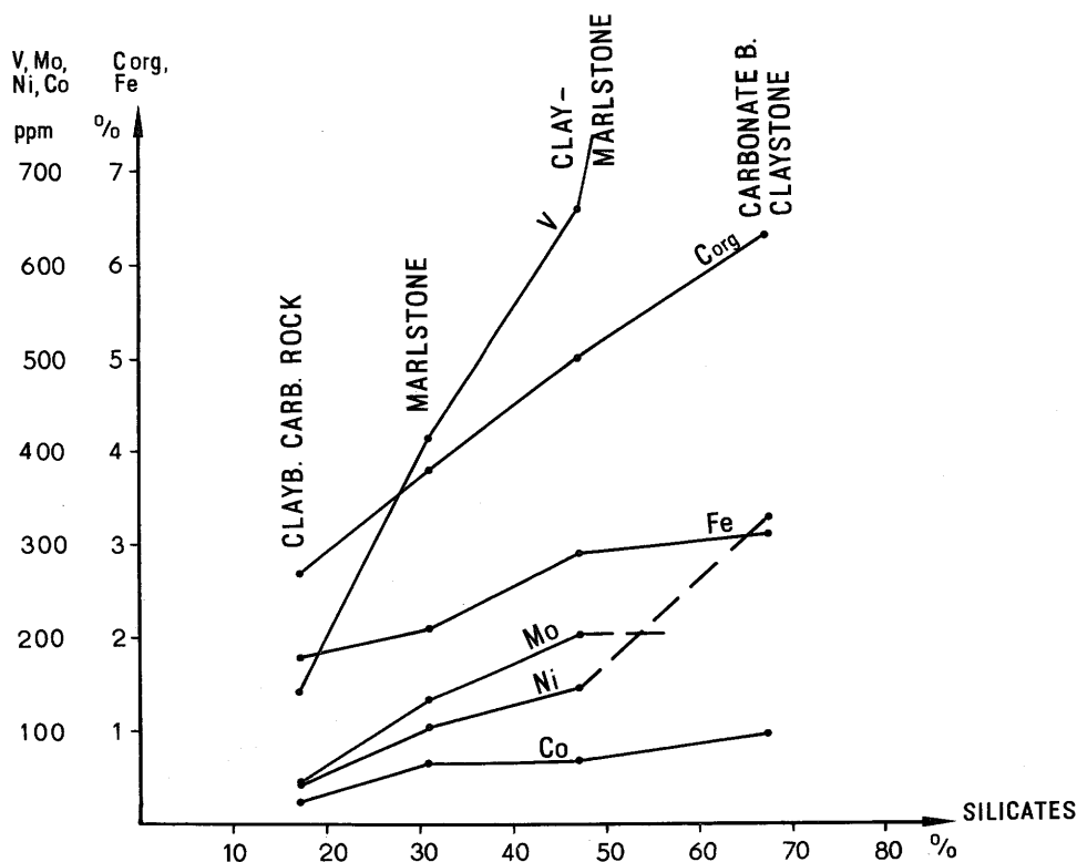
FIG. 5. — Correlation between the rock types of the Kupferschiefer and the C_{org} , Fe, V, Mo, Ni, and Co content.
